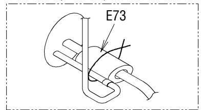
Z部詳細 (Detail Z)
