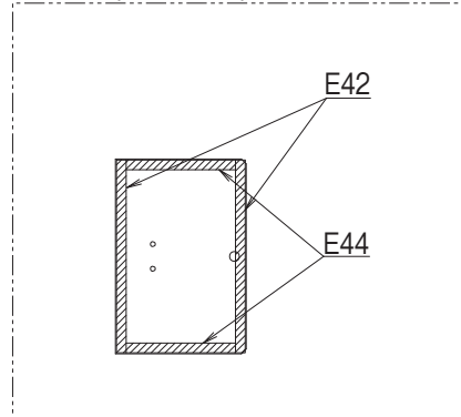
矢視AB(View AB)
