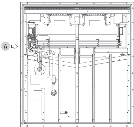
矢視A(View A)
